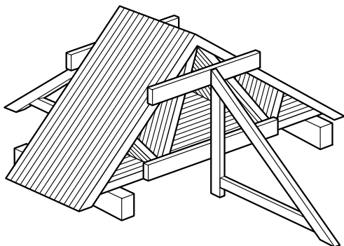
Trussed rafters: vertical stack before covering
